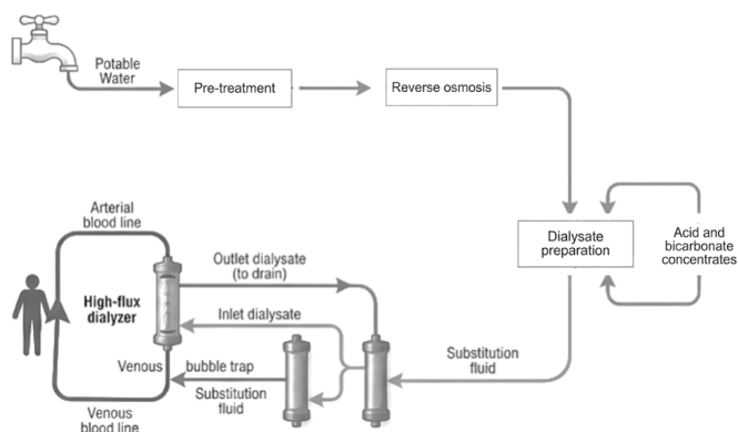
Figure 1. Diagram shows a typical flow for an HDF set-up and an example system
